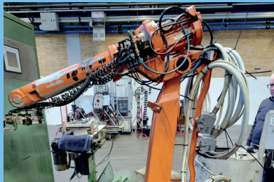
Riello Rotary Transfer Centre
